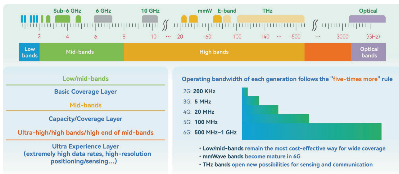
Figure 12 Multilayered frequency band framework
