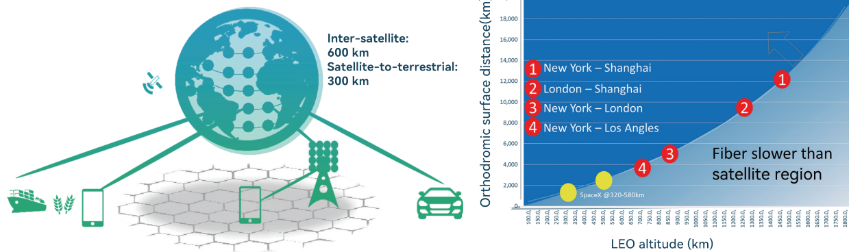
Figure 8 Integrated NTN for low-latency long-distance communication
